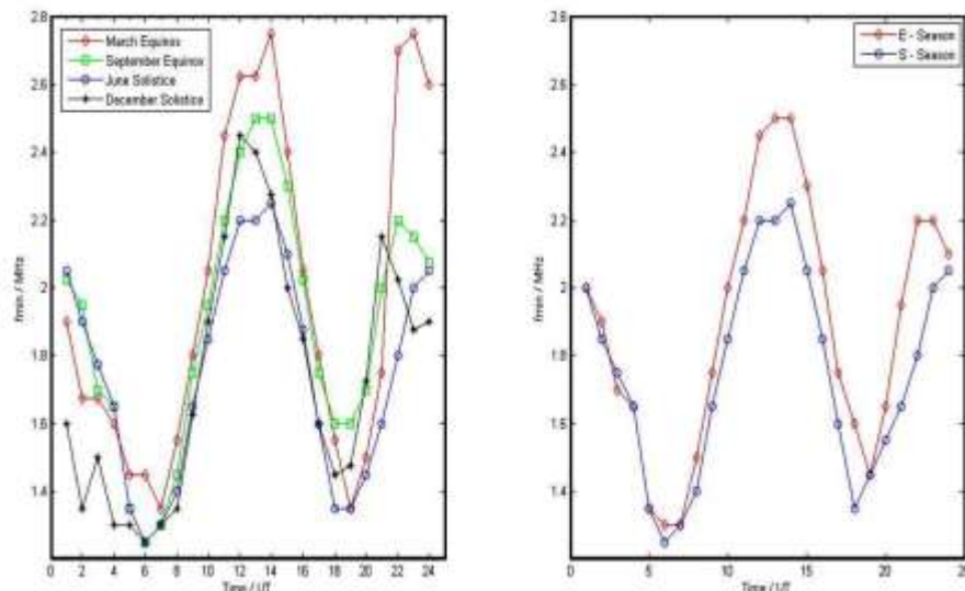
Figure 3: Seasonal variation of the ionospheric minimum frequency ( f_{min} ) obtained from the Digisonde. (a) Seasonal variation in f_{min} during the March equinox, September equinox, June solstice, and December solstice. (b) The comparative behaviour between the equinox season (E-season) and the solstice season (S-season).
